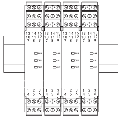
Vertically installation
