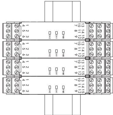
Vertically installation
