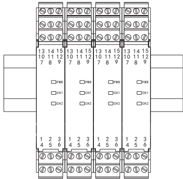
Horizontally installation
