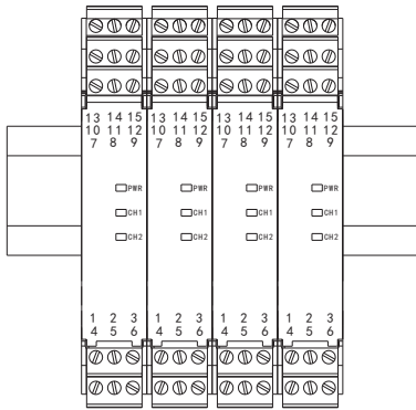
Horizontally installation
