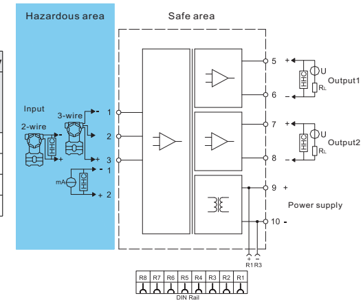
Single input, double output
